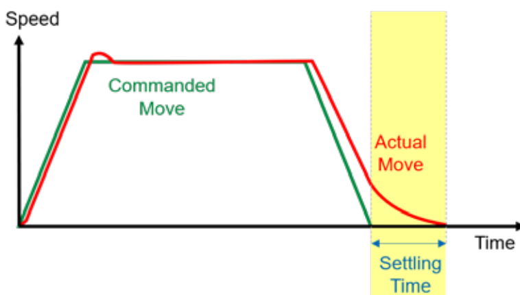
Figure 8: Settling Time of Actual Move
