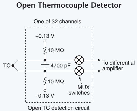
Fig. 6.11. The thermocouple provides a short-circuit path for dc around the capacitor, preventing it from charging through the resistors. When the thermocouple opens, due to rough handling or vibration, the capacitor charges and drives the input amplifier to the power supply rails, signaling a failure.
