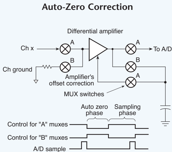
Fig. 6.10. Auto-Zero Correction compensates for analog circuitry drift over time and temperature. Although small, the offset could approach the magnitude of the thermocouple signal.
