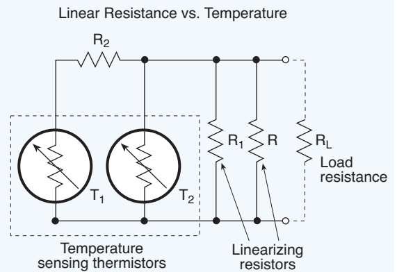
Fig. 6.23. Compensating resistors in the network linearize the resistance change vs. temperature in the same manner as they do for the voltage mode.
