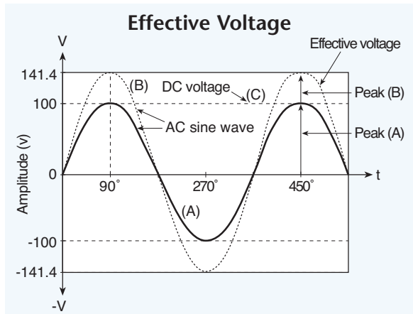
Fig. 4.03. The numerical value for the peak voltage of ac must be 1.414 times that of dc to produce the same heating effect.
