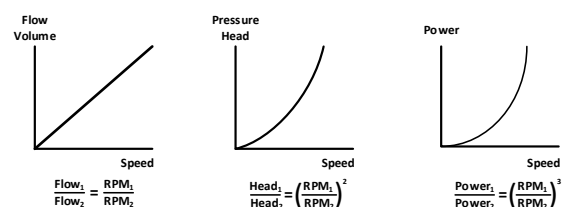
Figure 5. Affinity laws
